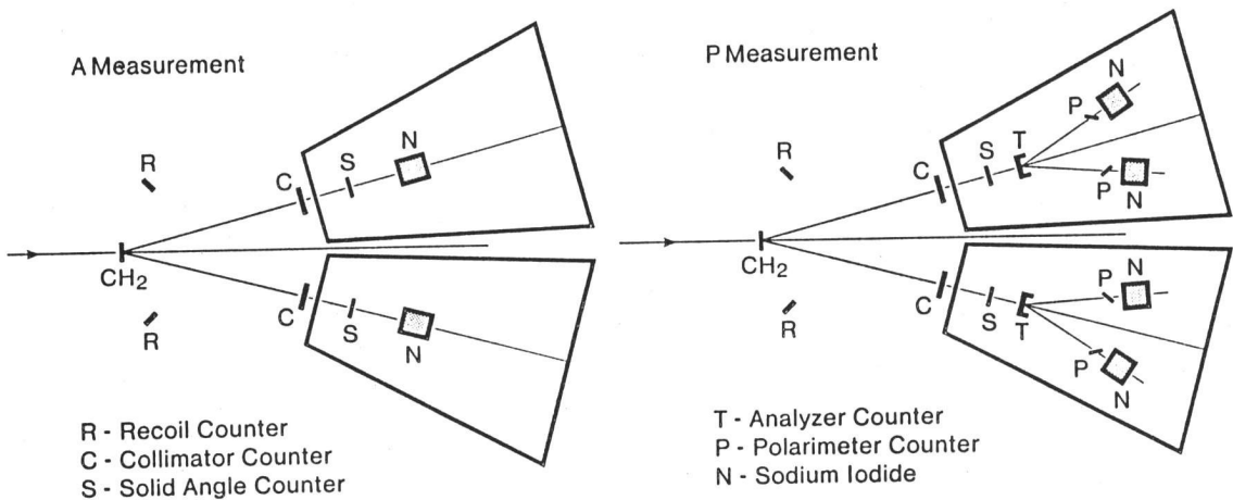
Fig. 1 Schematic layouts of apparatus for A and P measurements (not to scale)
