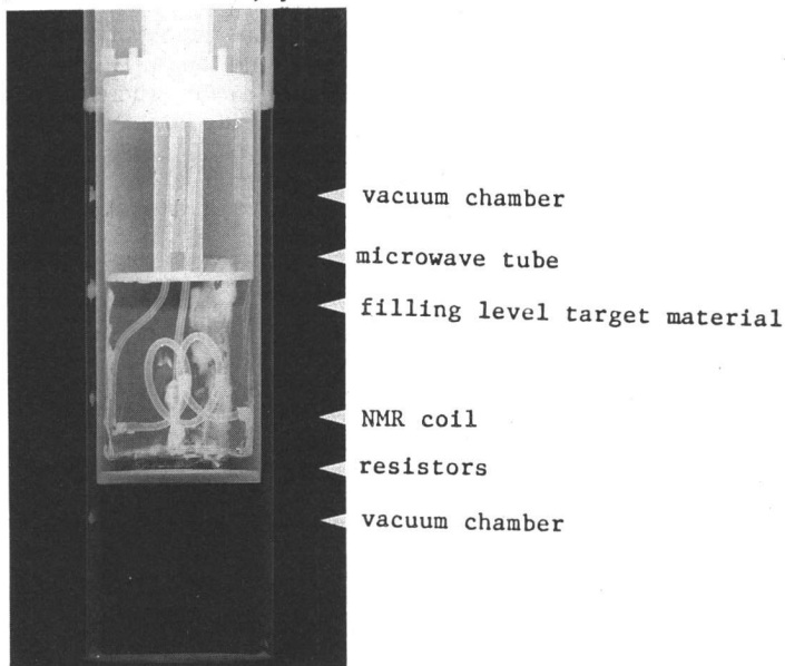
Fig. 1 X-ray of the target chamber.
